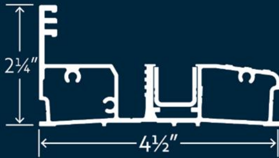
STANDARD SILL Water-Rated, Impact-Rated
