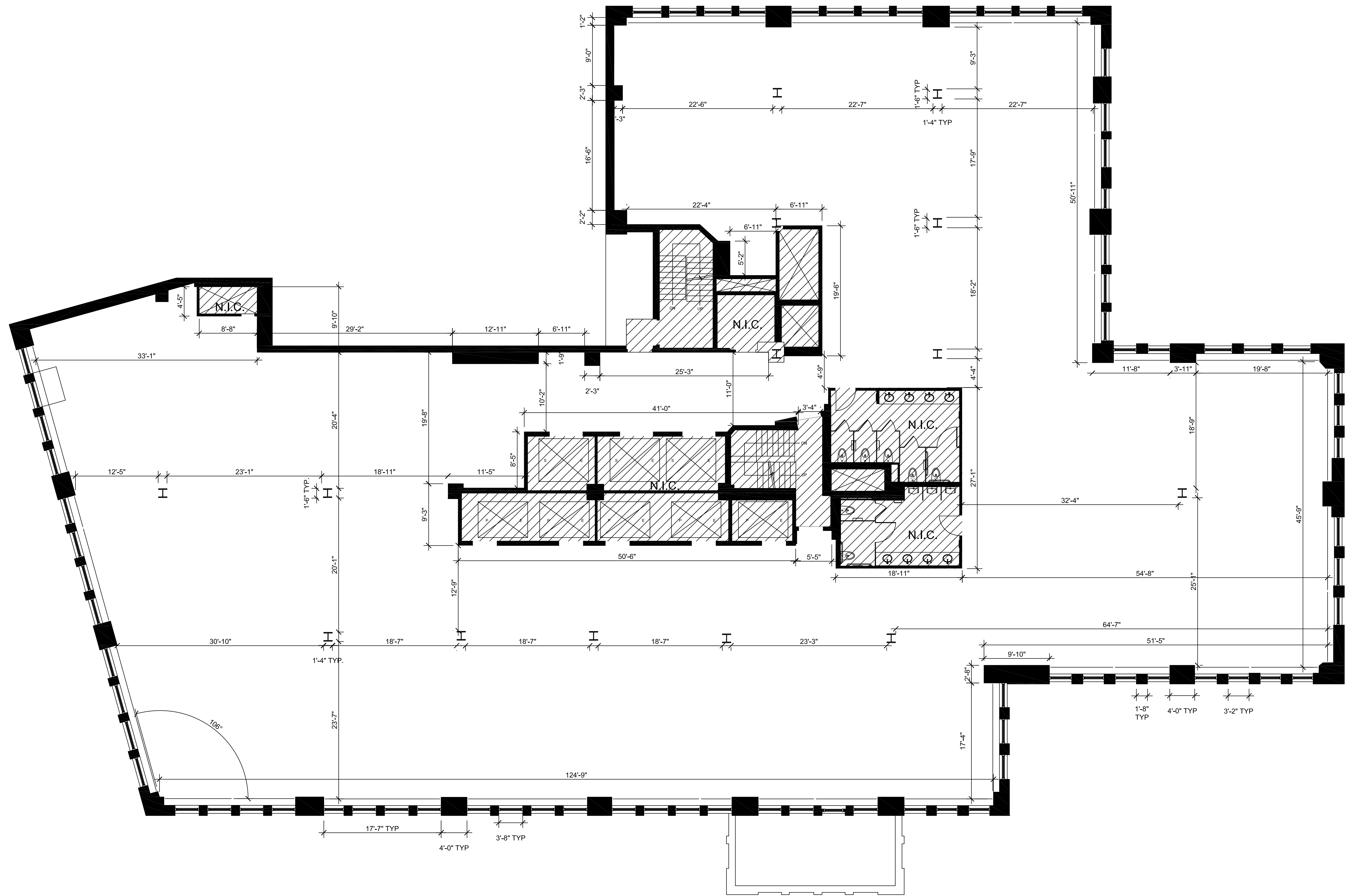
FLOOR PLAN SCALE 1/8" = 1'-0" CEILING HT: 12' AFF
